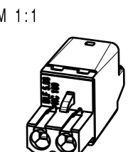
BLF 5.08/02/180 (Standard)
