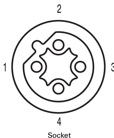
Straight socket
