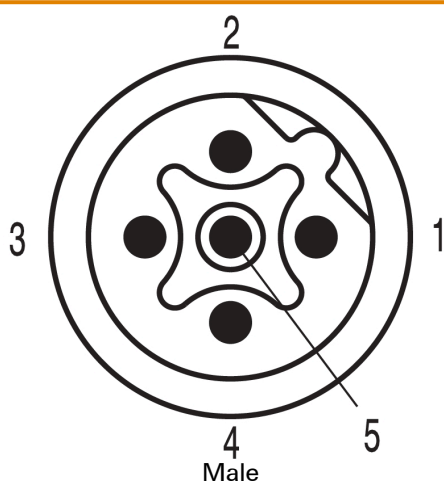
Male, angled
