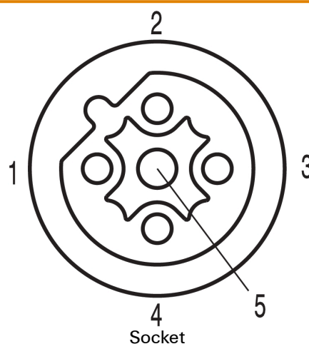
Straight socket
