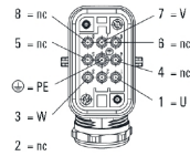
Pin assignments
