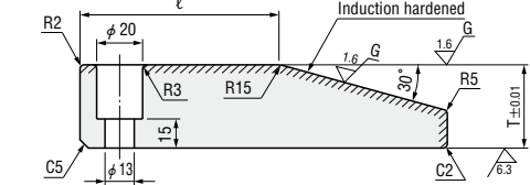
■ Shim for cam dwell wear plates
