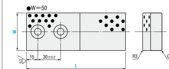
CS15W (Copper alloy type)
