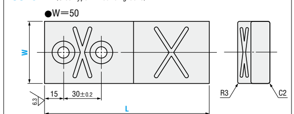
CS15F (Steel type) CS15FN (Steel type without oil groove)
